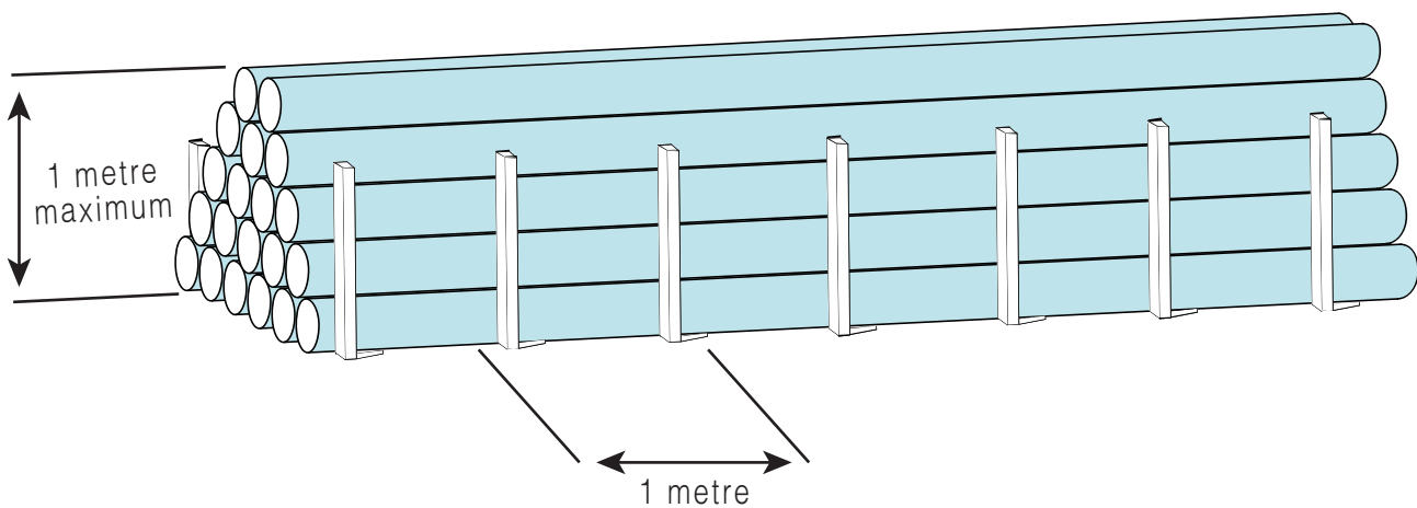
Storage of Loose pipes
